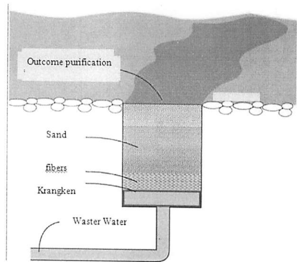
Figure 3. Wastewater filtration
